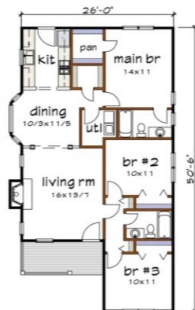
Floor 1 plan
